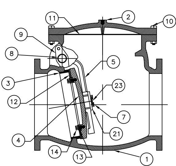
14"-30" CHECK VALVE BODY
