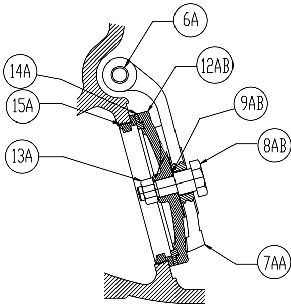
4'-12" PLAIN CHECK BRONZE SEATED DISC ASSEMBLY
