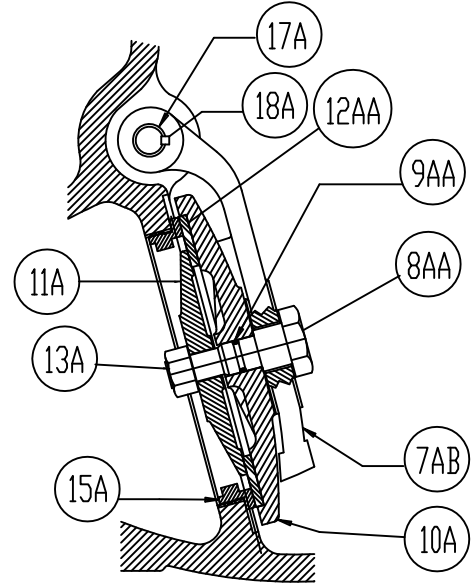
4'-12' LEVER & WEIGHT RESILIENT SEATED DISC ASSEMBLY
