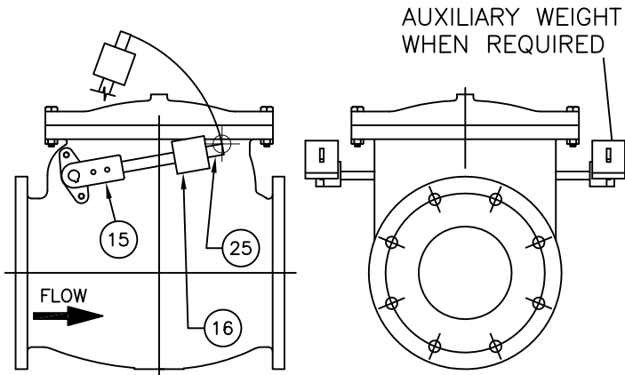
LEVER & WEIGHT CHECK VALVE
