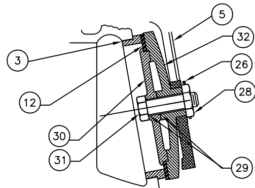
14" CLAPPER ASSEMBLY
